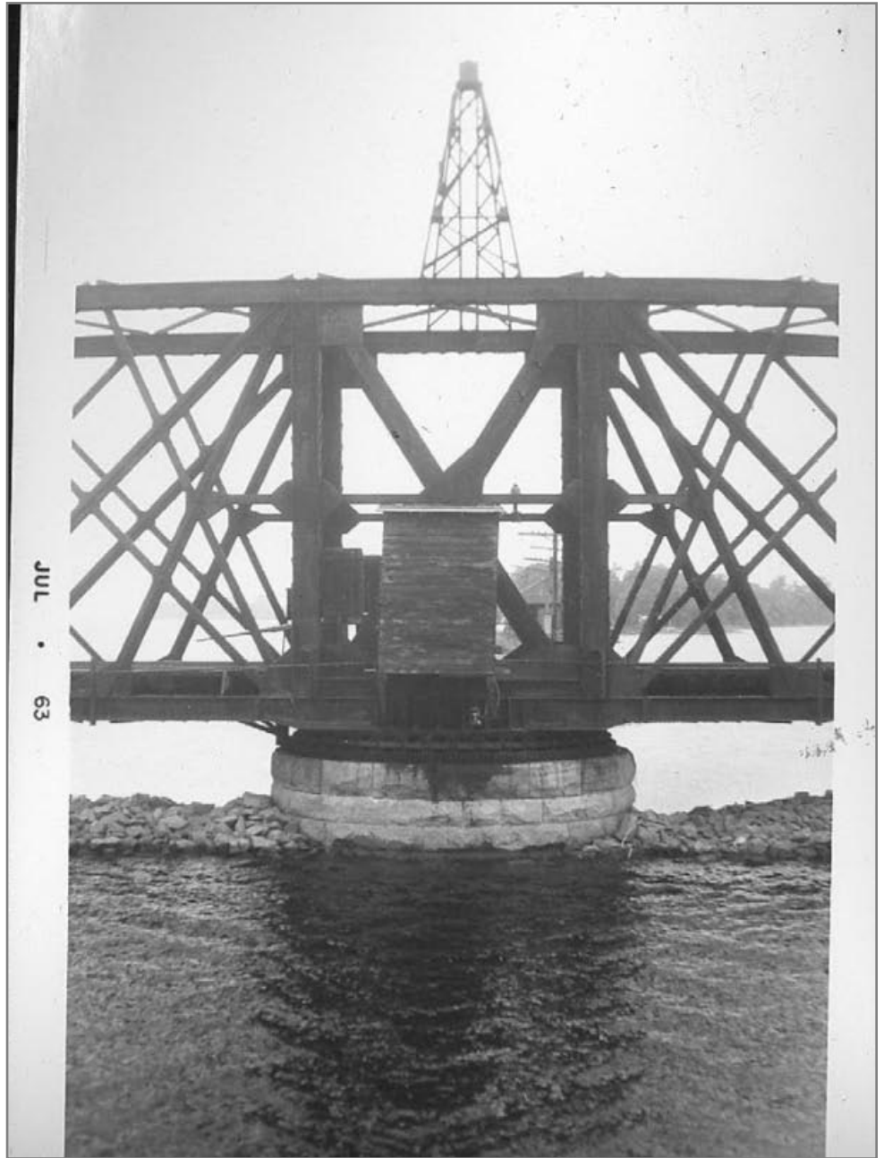
Bridge 275 Northbound 6/29/63
