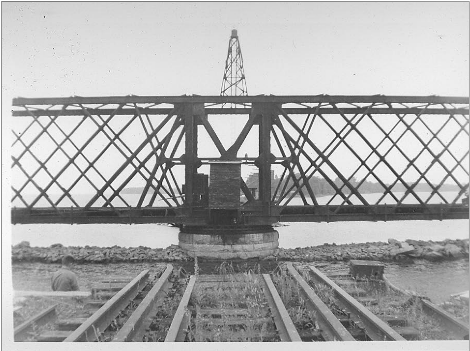
Bridge 275
